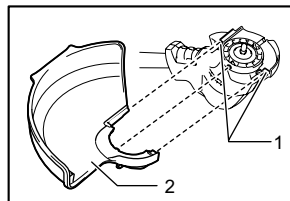
1. Grooves 2. Protector
